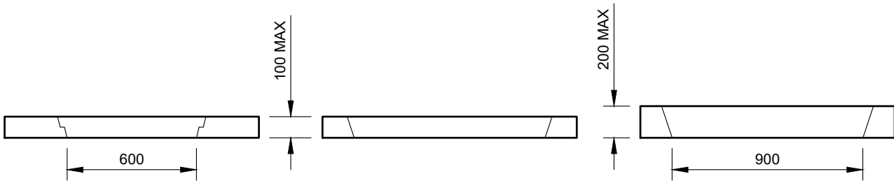
SECTION VIEW CLASS B
