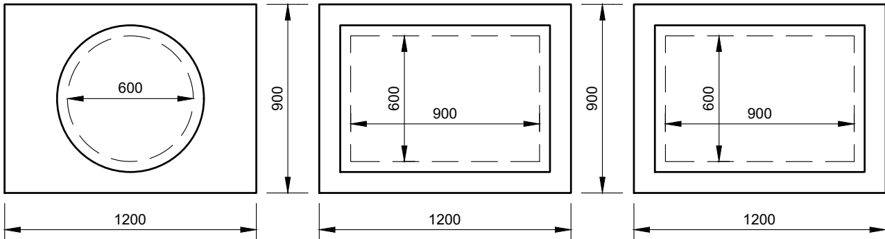
CLASS B JUNCTION PIT COVER PLAN
