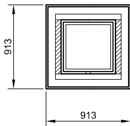
PLAN OF SURROUND
