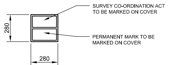
COVER DETAILS
