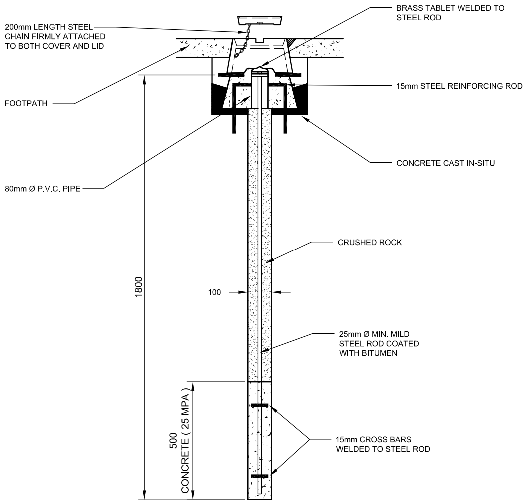
SECTIONAL VIEW
